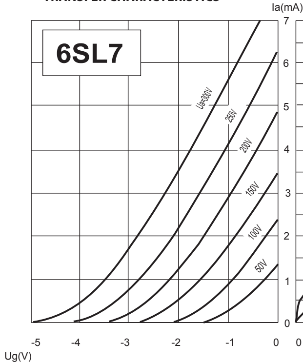
TRANSFER CHARACTERISTICS
